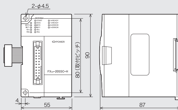
FX3U-20SSC-H 質量: 0.3kg
