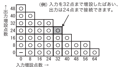
FX2N-48ER-UA1/UL
