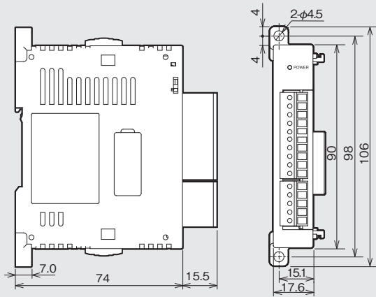
FX3U-3A-ADP, FX3U-4AD-ADP, FX3U-4DA-ADP, FX3U-4AD-TC-ADP, FX3U-4AD-PT-ADP, FX3U-4AD-PTW-ADP 質量: 0.1kg
