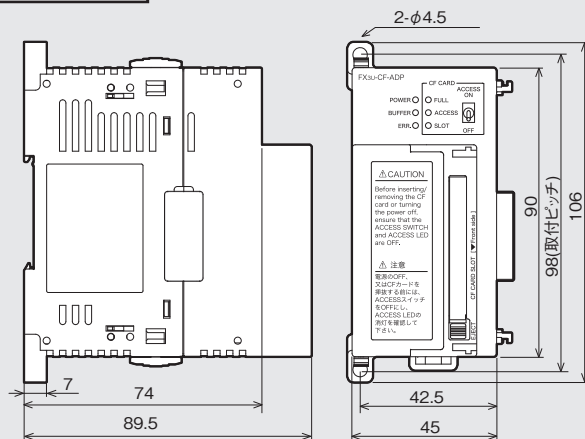
FX3U-CF-ADP
