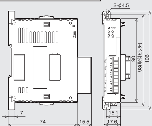
FX3U-4HSX-ADP, FX3U-2HSY-ADP
