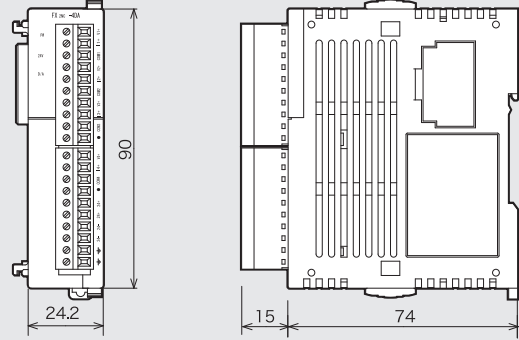
FX2NC-4DA
