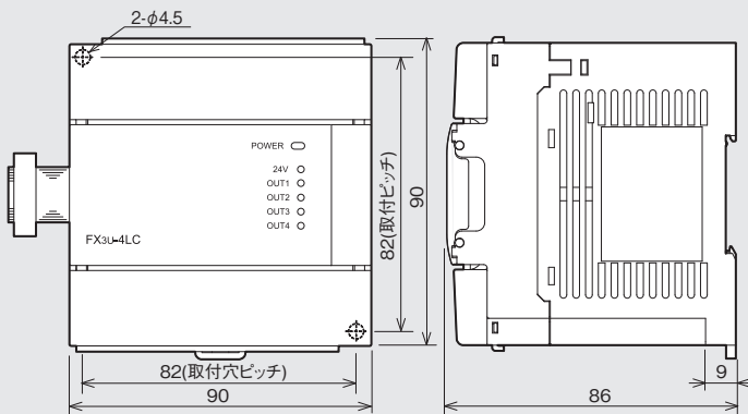
FX3U-4LC
